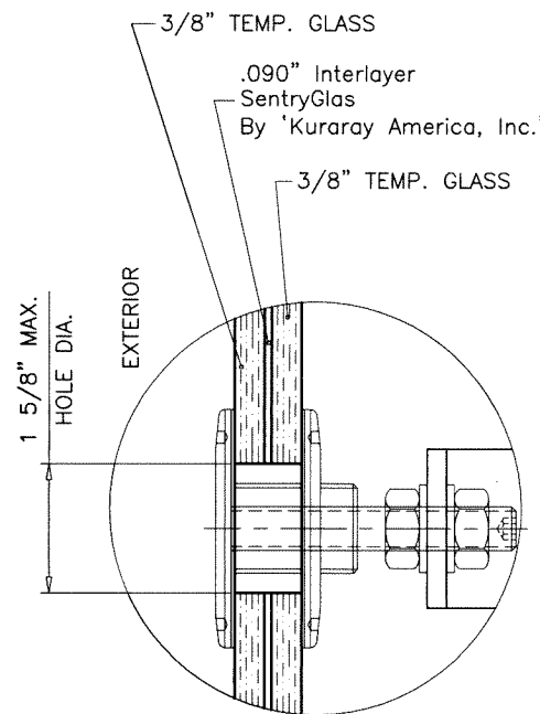
GLASS TYPE 'B' 13/16" OVERALL NOMINAL THK.
