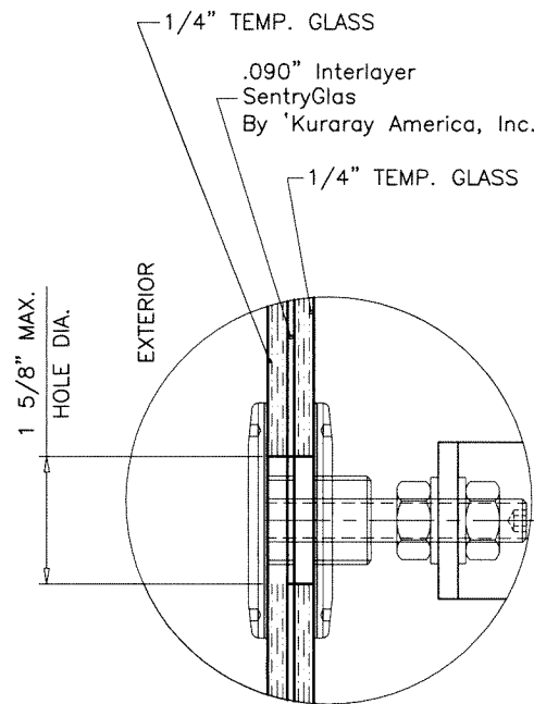
GLASS TYPE 'A' 9/16" OVERALL NOMINAL THK.
