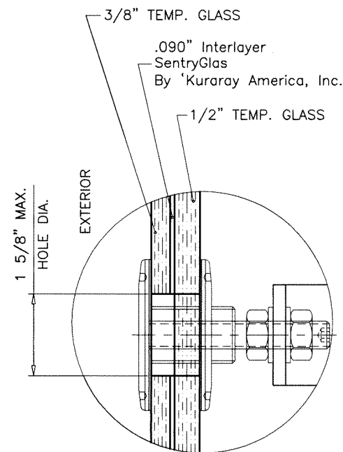
GLASS TYPE 'C' 15/16" OVERALL NOMINAL THK.
